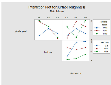
Fig 6. Surface unevenness Interaction plot
