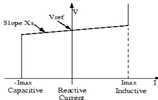
Fig 3. V-I Characteristics STATCOM
