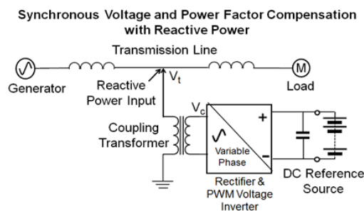
Fig 2 Transmission Line STATCOM
