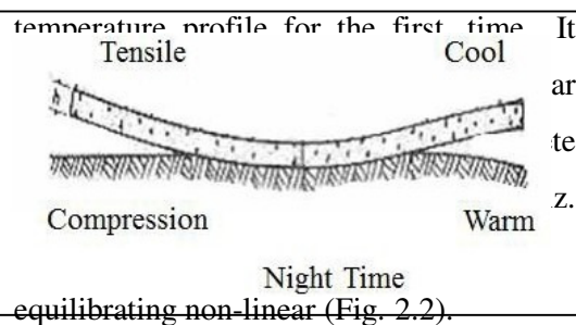
Fig. 2.2: Stress components due to non-linear temperature profile (Siddique et al. 2005, Hiller et al. 2010)
