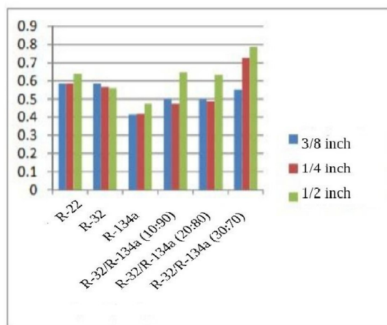
Graph: 2 Variation of Compressor Power with Blinding Ratio Refrigerant R-22, R-134a, R-32, R-32/R-134a
