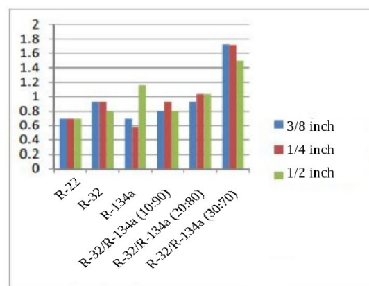
Graph: 1 Variation of Refrigeration Effect with Blinding Ratio Refrigerant R-22, R-134a, R-32, R-32/R-134a
