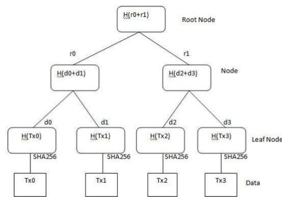
Figure 1.2: Merkle Tree
