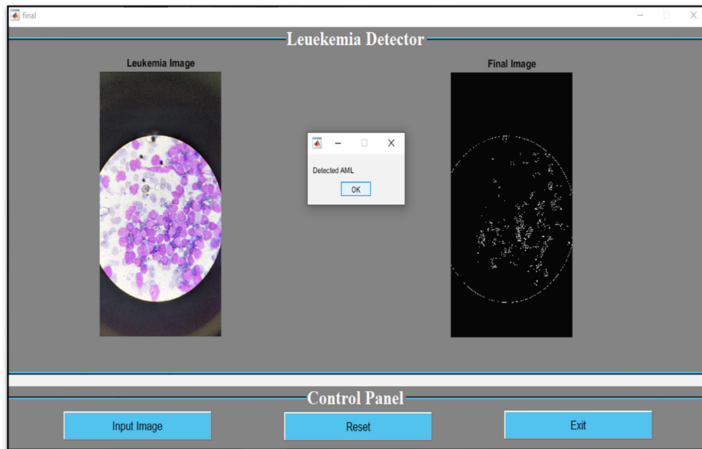
Fig.2.Detected AML
