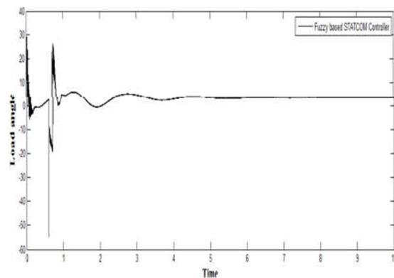
Fig.18 Load angle with time (after clearing fault)
