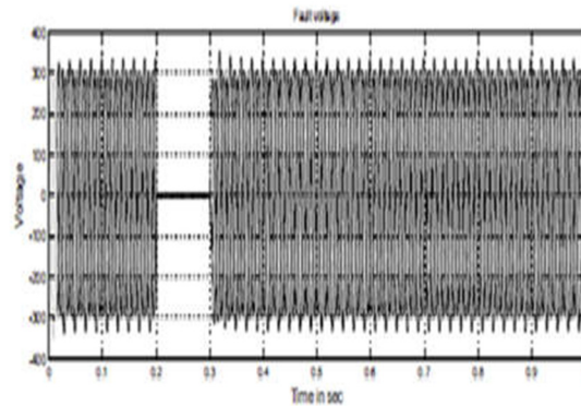
Fig.19 Three Phase Fault Voltage
