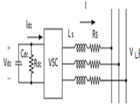
Fig.1 STATCOM's Basic Circuit Diagram
