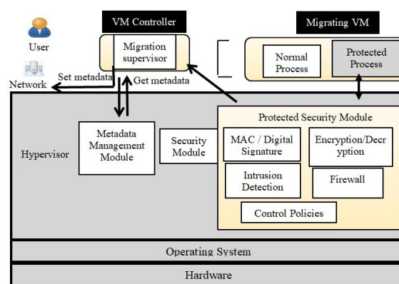
Figure 1: Protected Secure Live Migration
