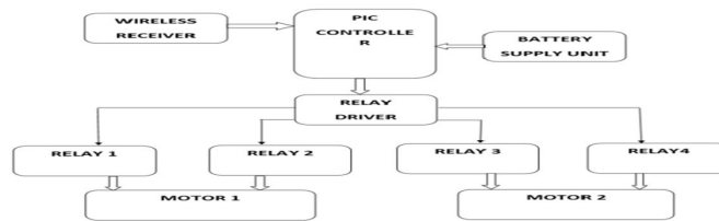
Fig 2: Block of receiver unit on wheelchair
