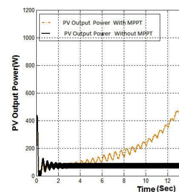
Figure 13 Output Current for the solar irradiance (1000 w/m 2 ) in hybrid MPPT technique
