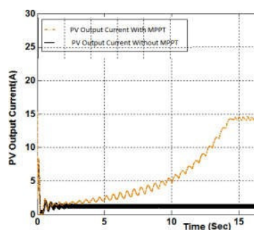
Figure 9 Output Current for the solar irradiance (600 w/m 2 ) in hybrid MPPT technique
