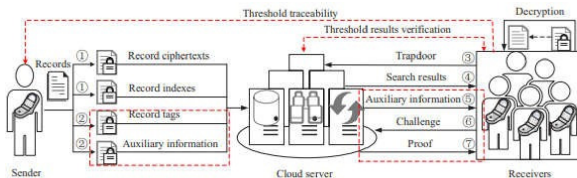
Fig 2: System Model
