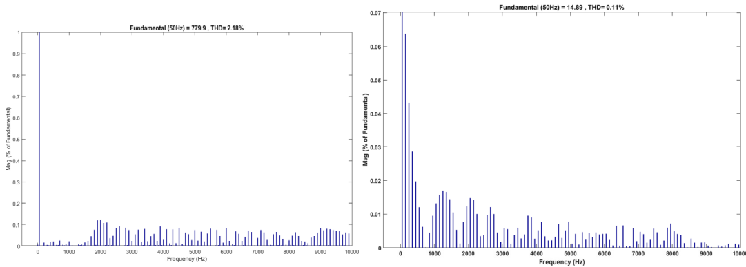
Fig.11 THD of output voltage and current with LS-PWM when modulation index is 1 and load is 50\Omega and 50mH
