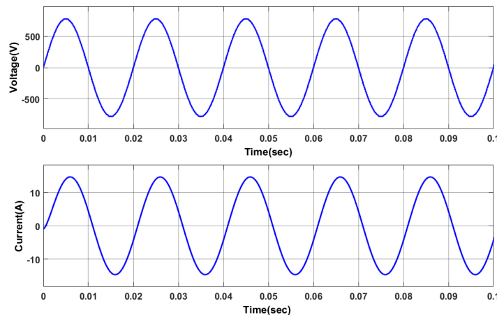
Fig.10 53 level inverter output voltage and current with Modified SHE-PSO with 50 \Omega and 50mH load
