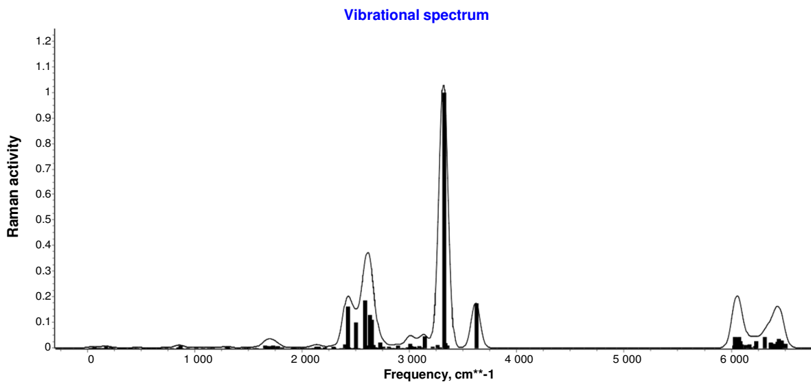
Figure 3: Raman activitty of 9CB molecule.
