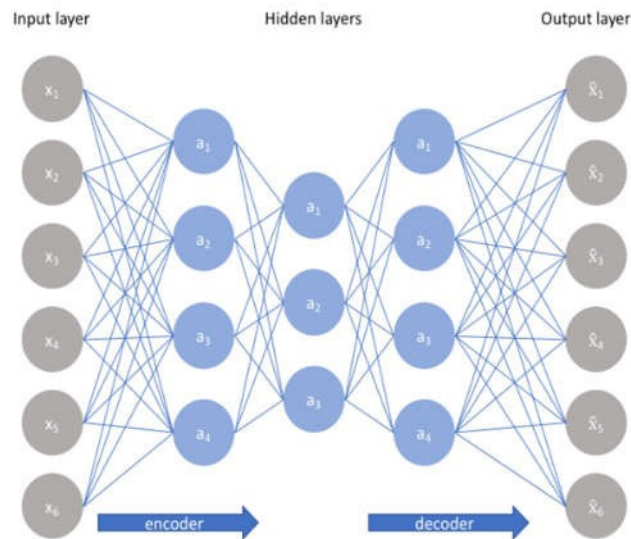
Figure 4. Autoencoder Model
