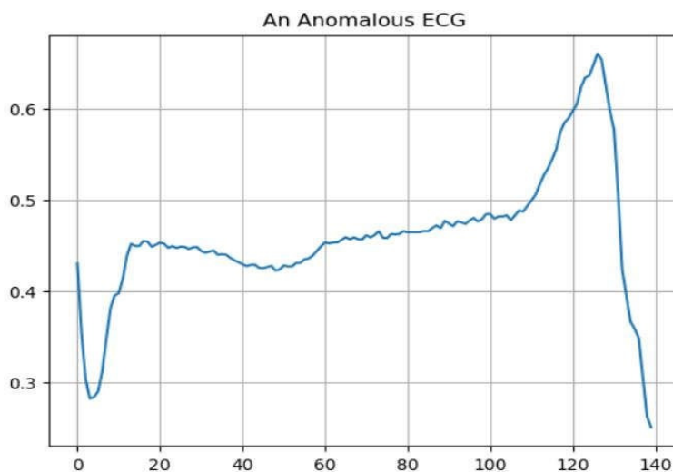
Figure 3. Anomalous ECG
