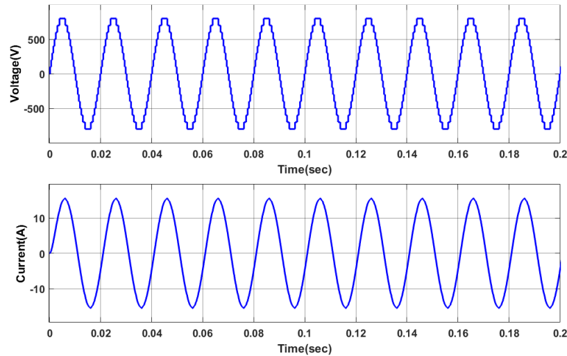
Fig.5 17 level inverter output voltage and current with Modified SHE with 50 \Omega and 50mH load
